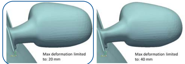
CAD Deformation According to Drag Sensitivity Map
