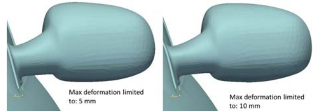
CAD Deformation According to Drag Sensitivity Map
